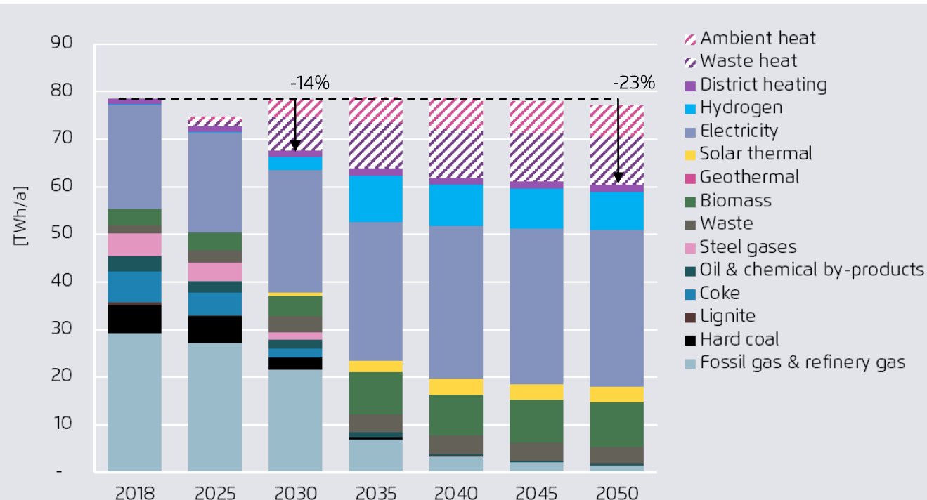
Final energy demand in industry in Romania
