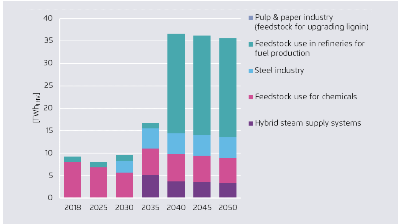
Net* hydrogen demand per sector and appliance in industry and refineries in Romania
