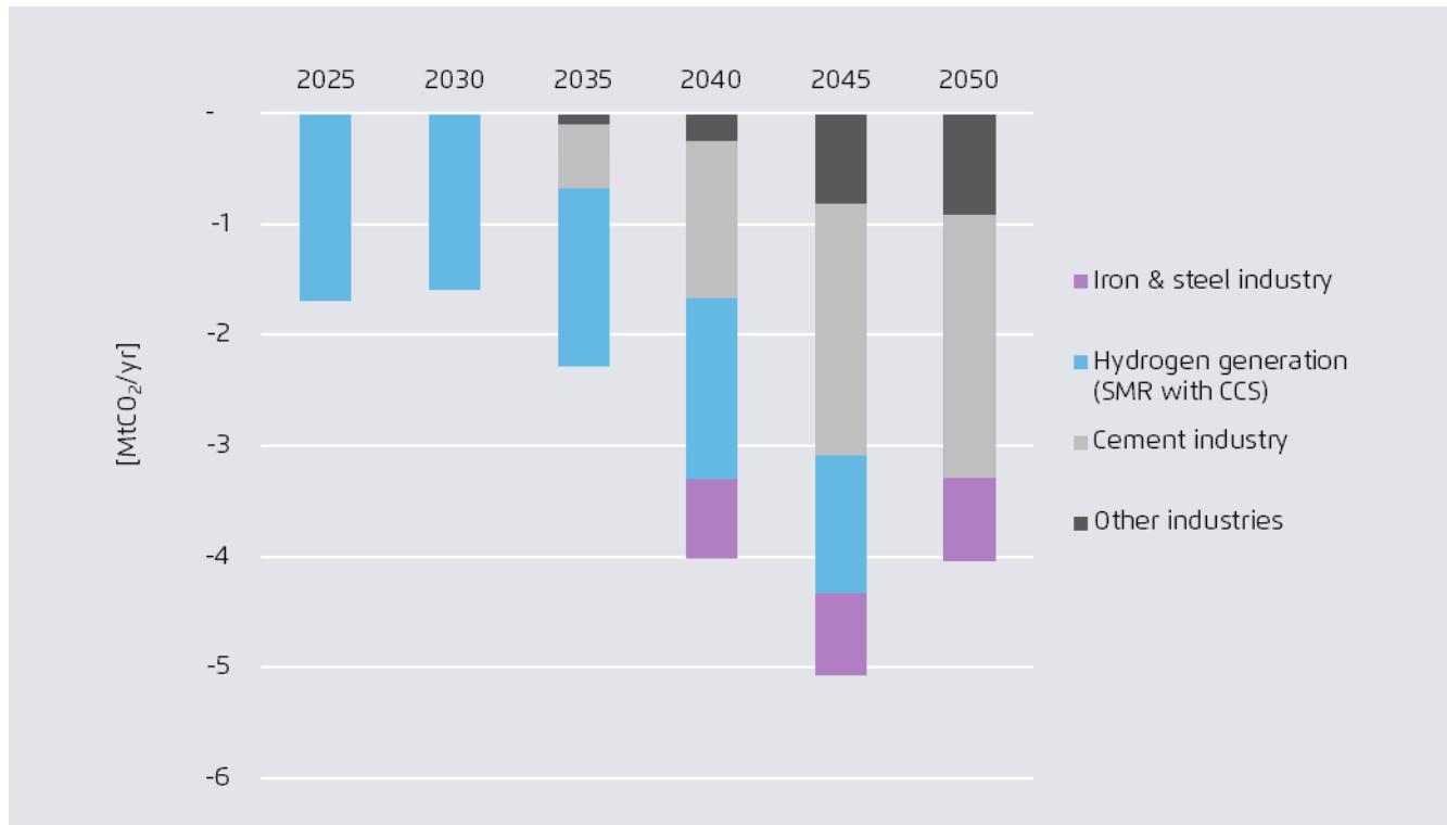
CCS balance in Romania's Gas Exit Pathway
