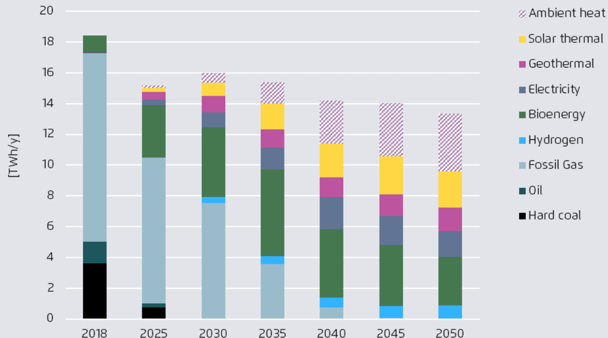
Energy input to district heating (including CHPs), Romania
