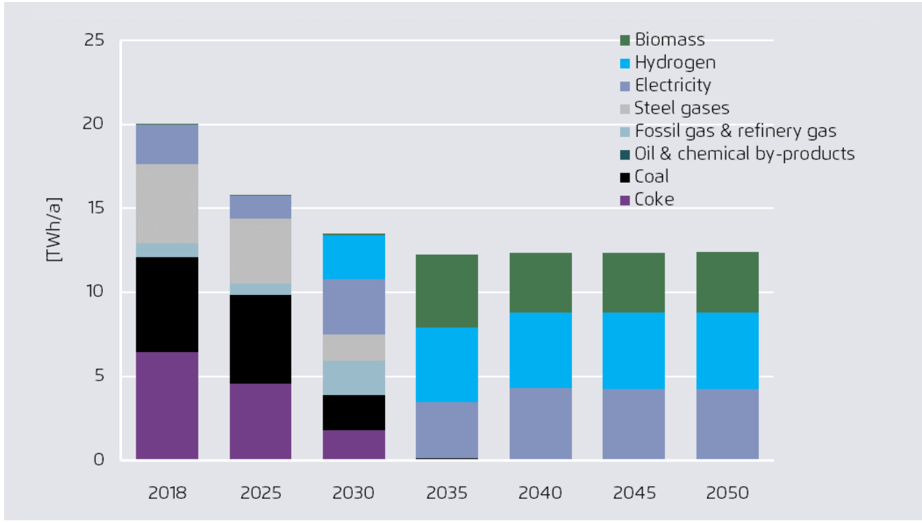
Final energy use of the steel industry, Romania
