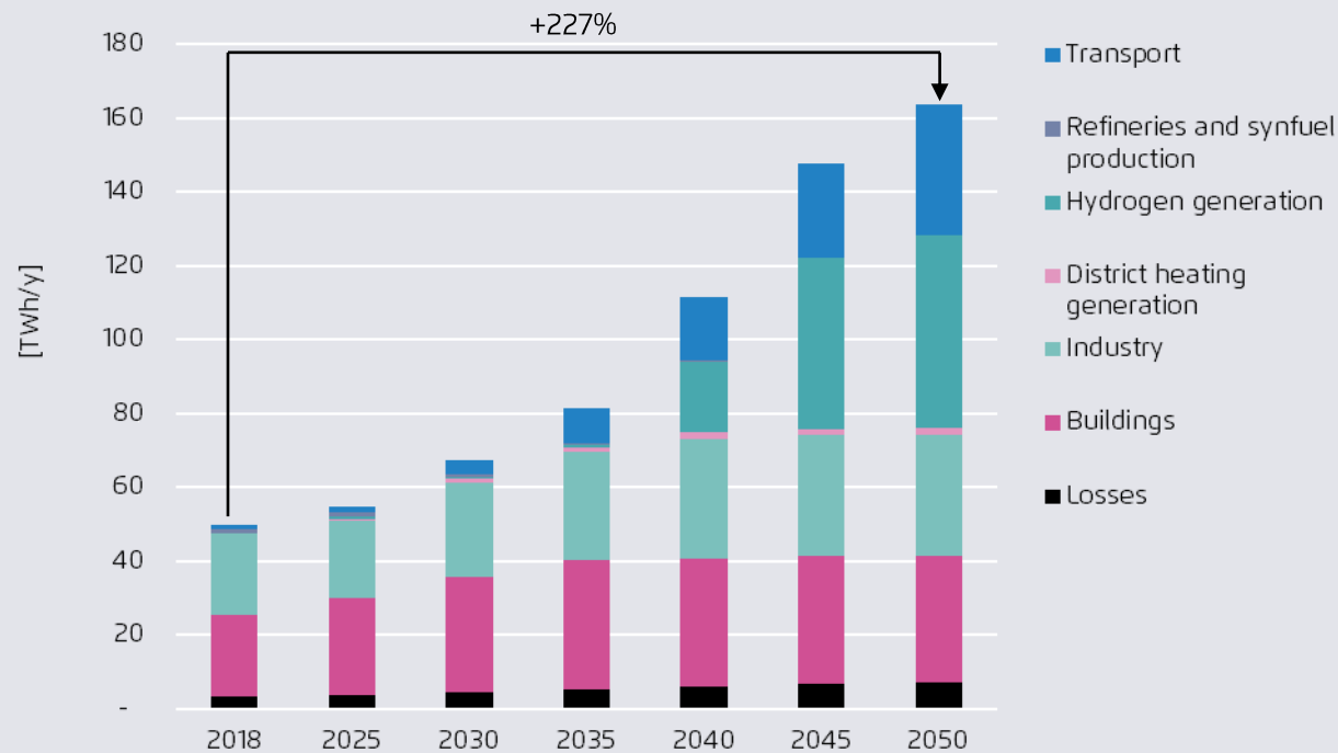
Power consumption by sector for Romania
