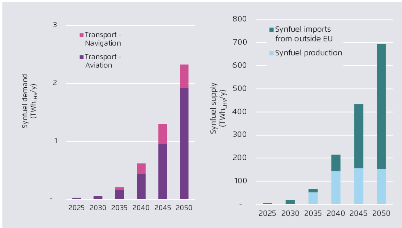
Synthetic fuel demand in Romania, and supply mix at EU-27 level
