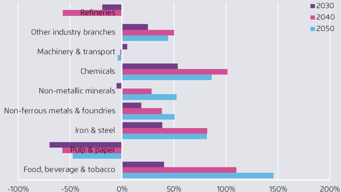
Gross power demand evolution compared to 2018 in the Romanian industry
