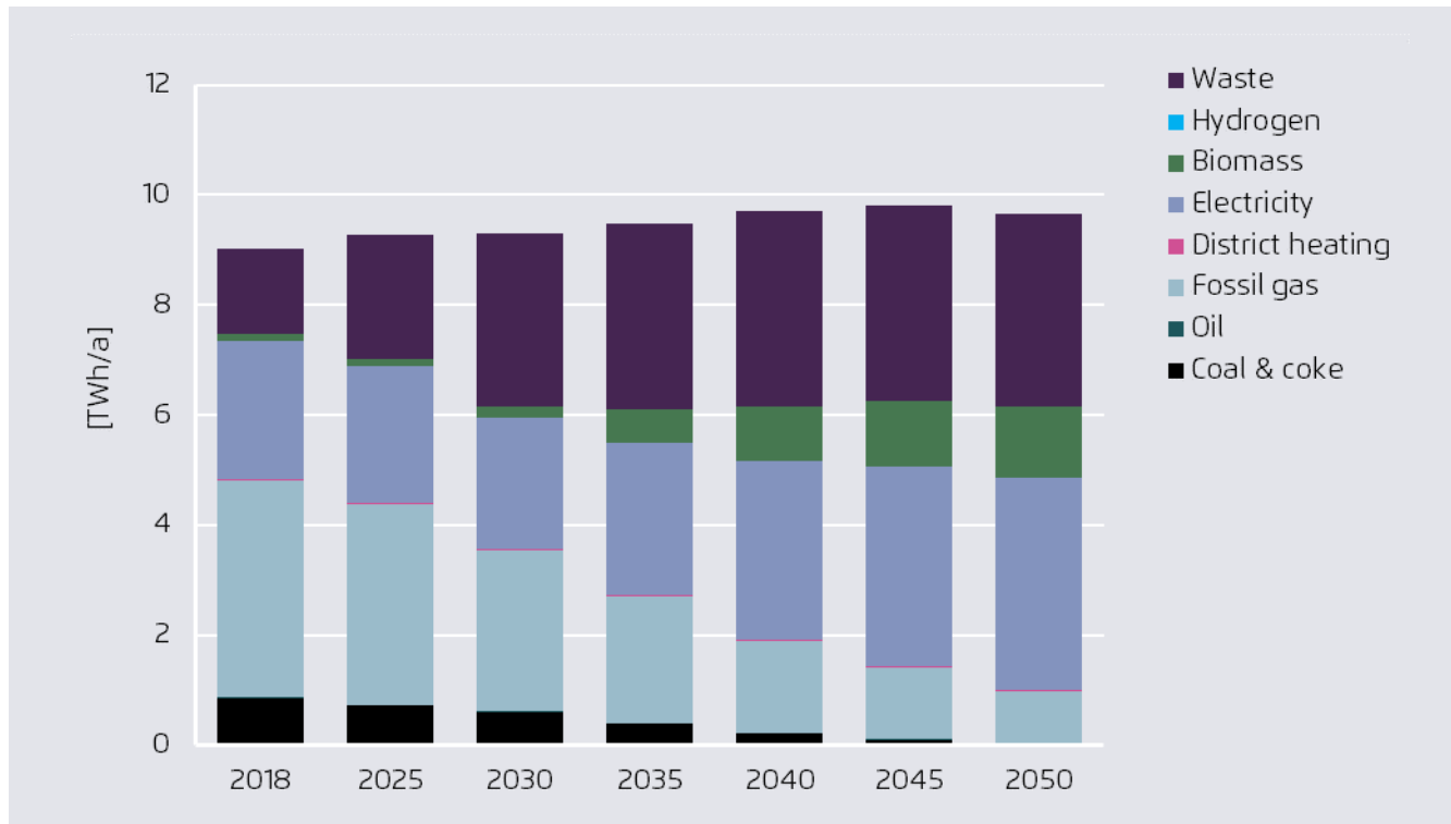
Final energy demand in the processing of non-metallic minerals, Romania
