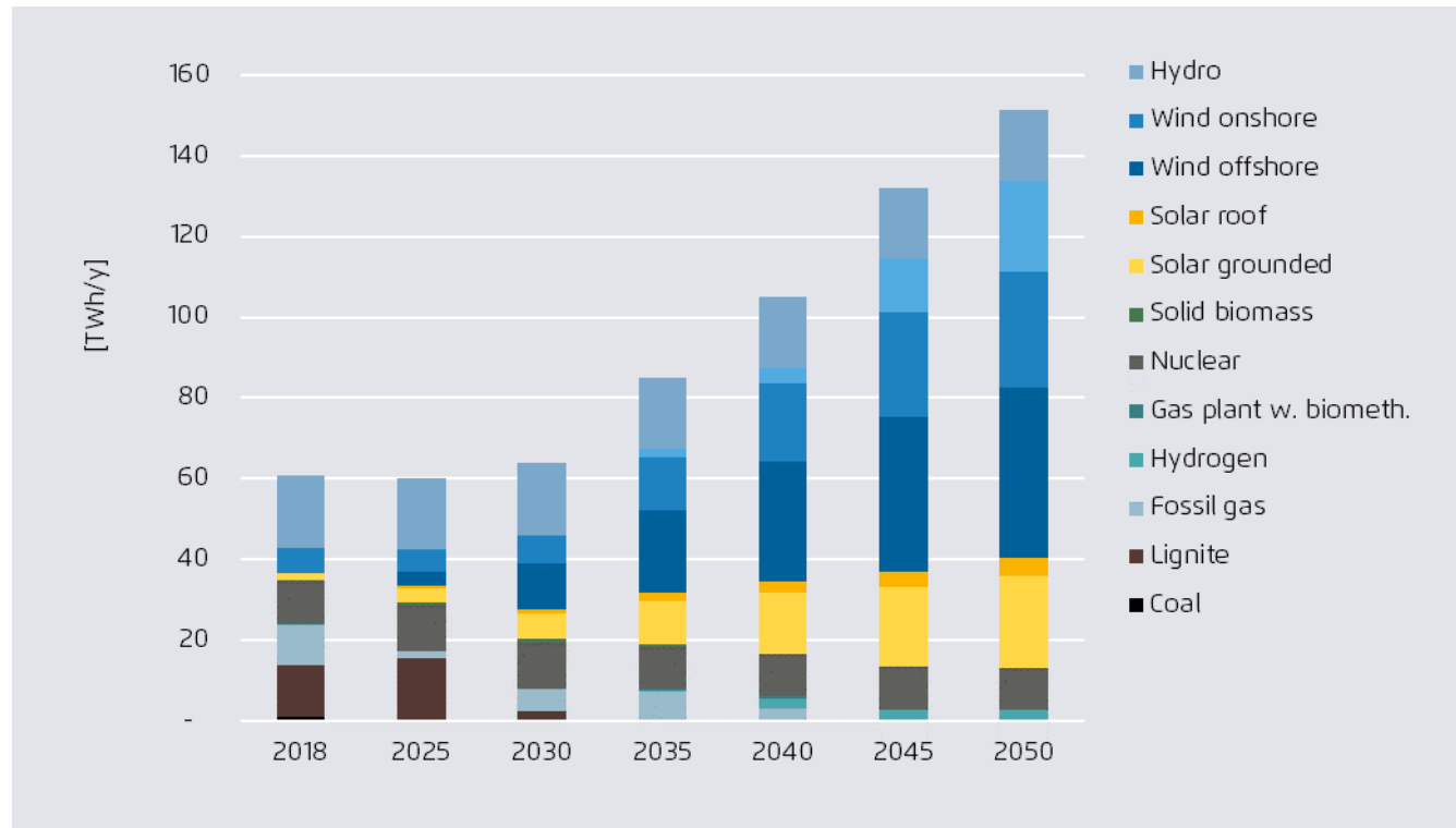
Power generation in Romania
