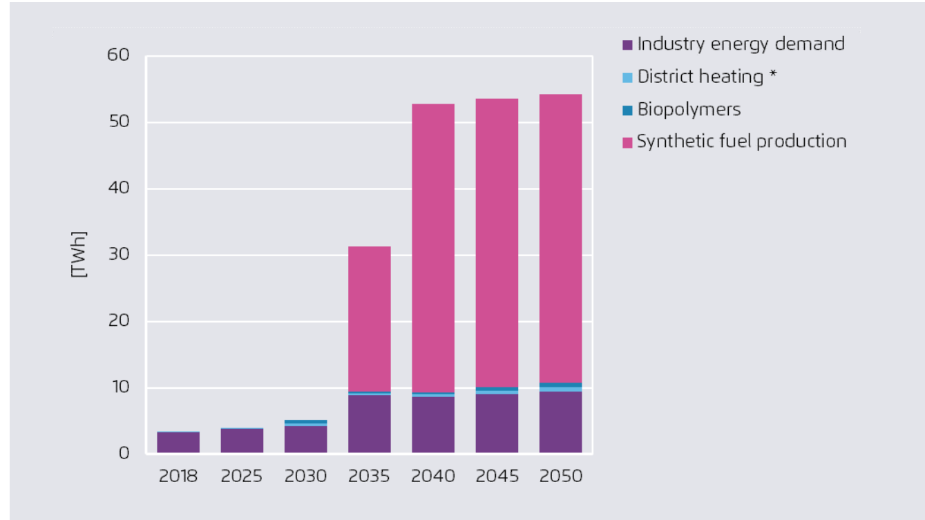
Biomass use for final energy, district heating and synthetic hydrocarbons, Romania
