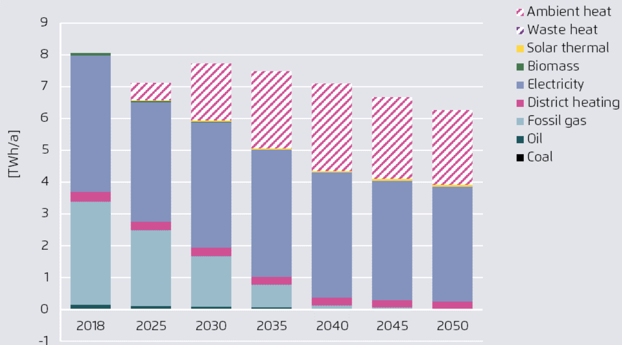
Final energy demand in machinery & transport equipment, Romania
