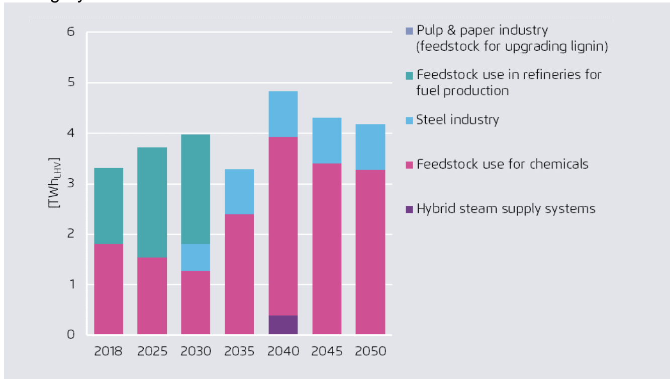
Net* hydrogen demand per sector and appliance in industry and refineries in Hungary
