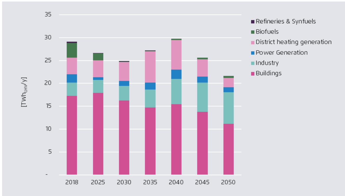
Energy and non-energy consumption of biomass by sector in Hungary
