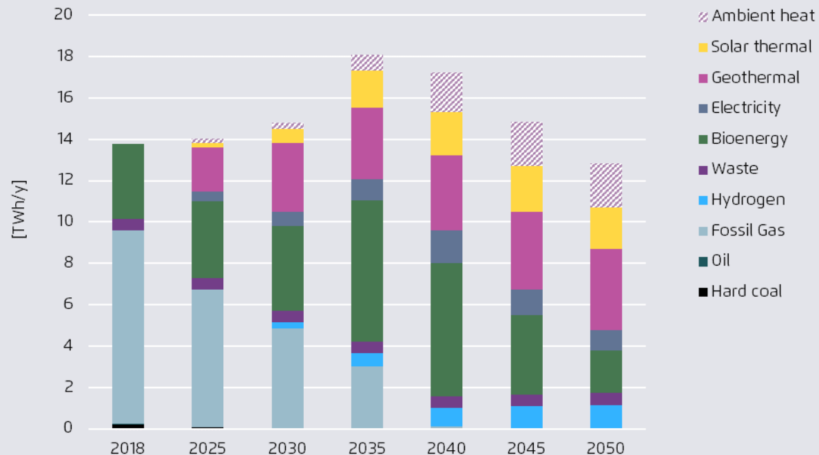
Energy input to district heating (including CHPs), Hungary
