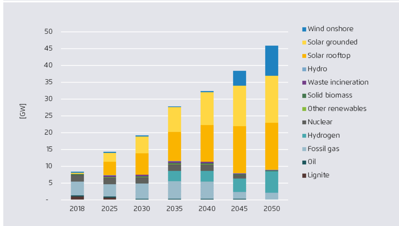
Power generation capacity, Hungary
