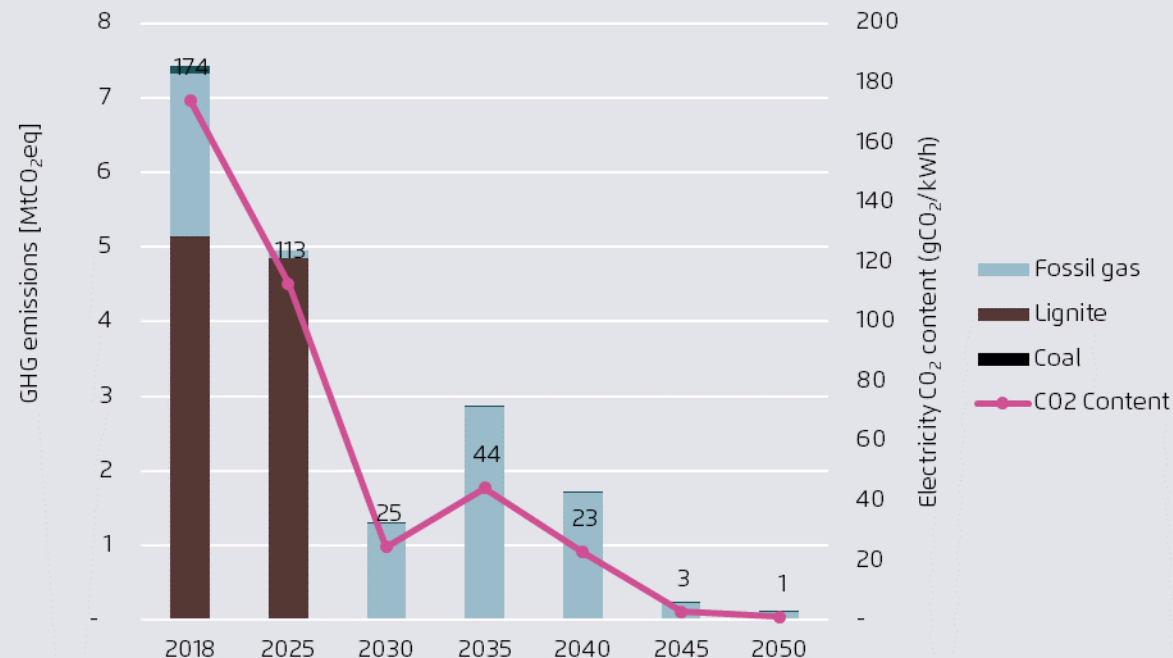
Evolution of electricity CO 2 content, Hungary
