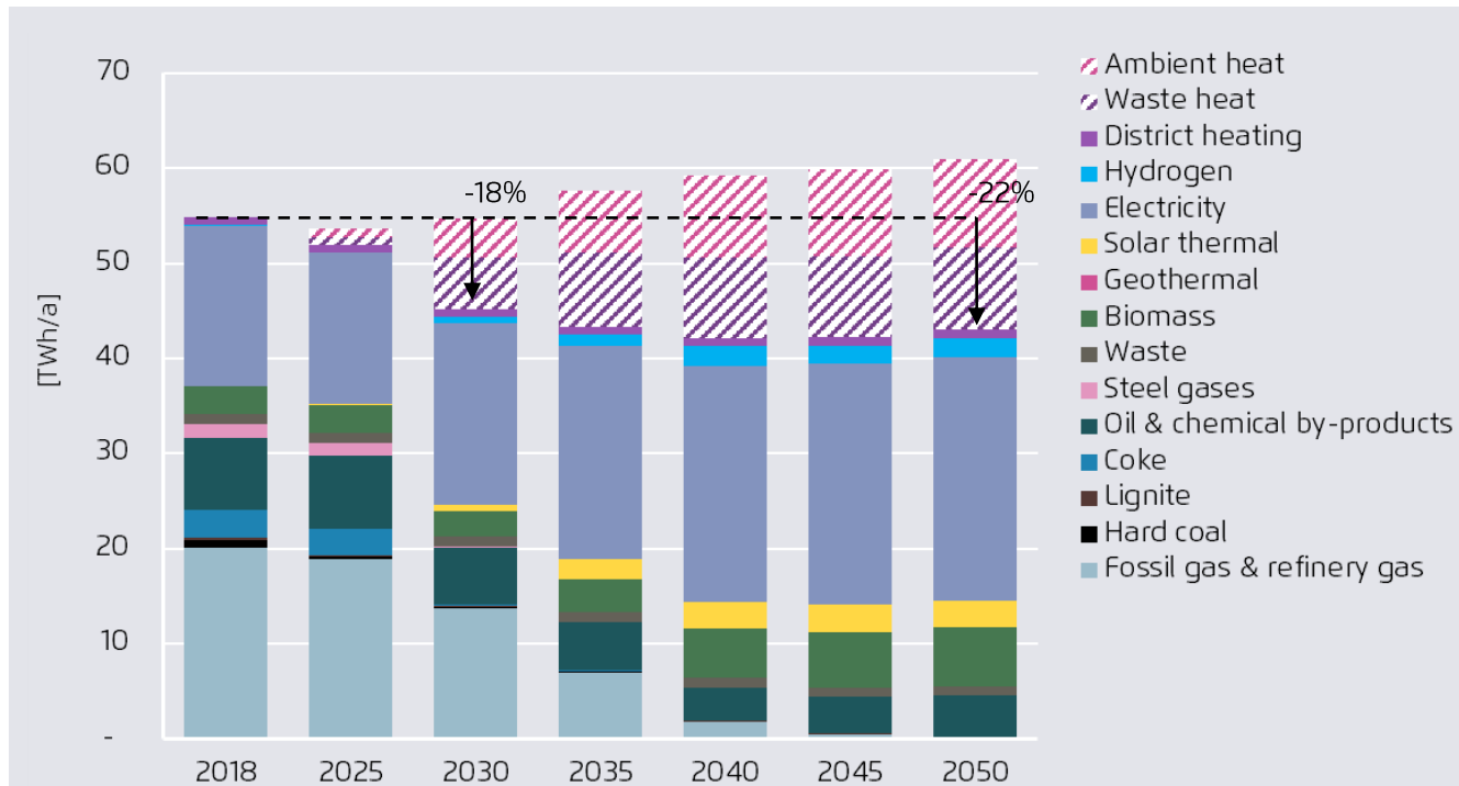
Final energy demand in industry in Hungary
