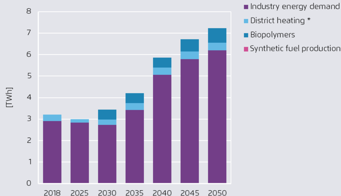
Biomass use for final energy, district heating and synthetic hydrocarbons, Hungary
