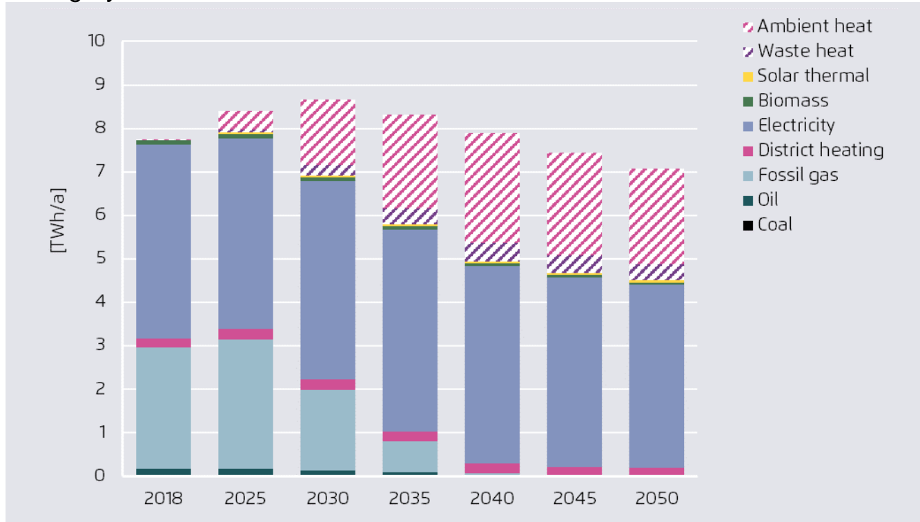
Final energy demand in the manufacturing of machinery & transport equipment, Hungary
