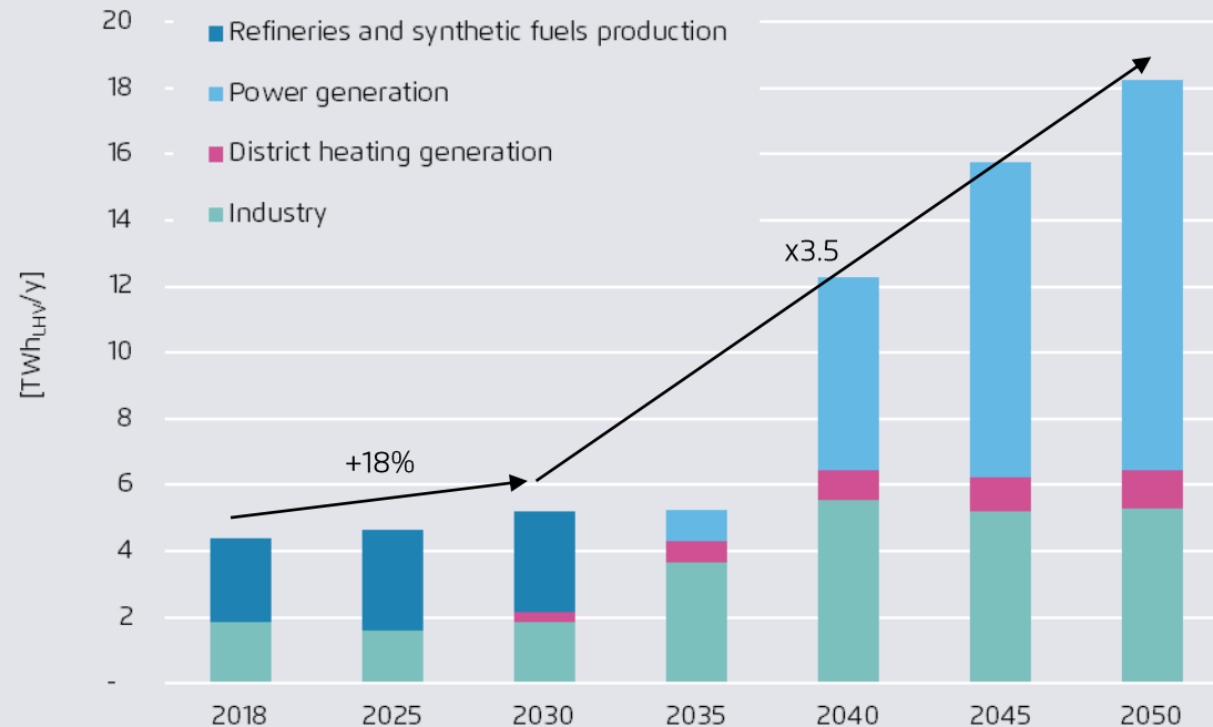
Hydrogen consumption by sector for Hungary
