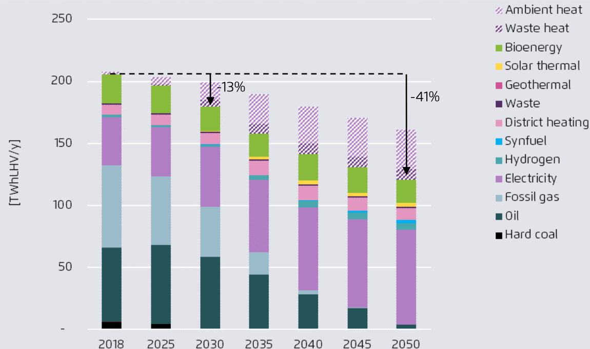
Final energy demand by energy carrier, Hungary
