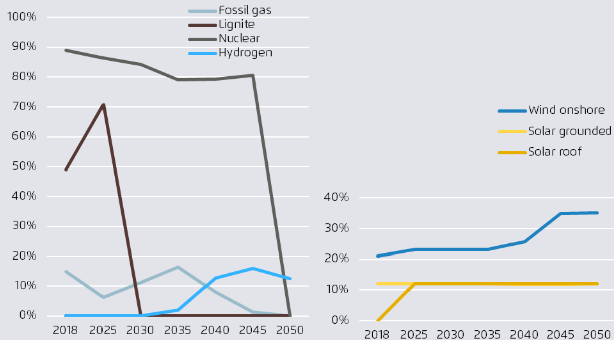
Capacity factor per technology (%)
