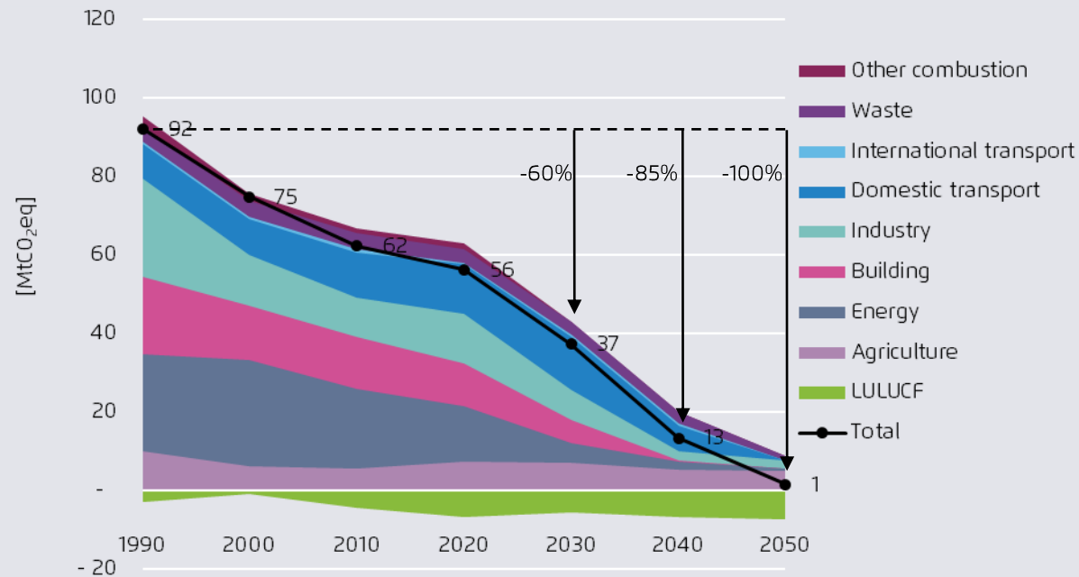
GHG emissions by sector in Hungary
