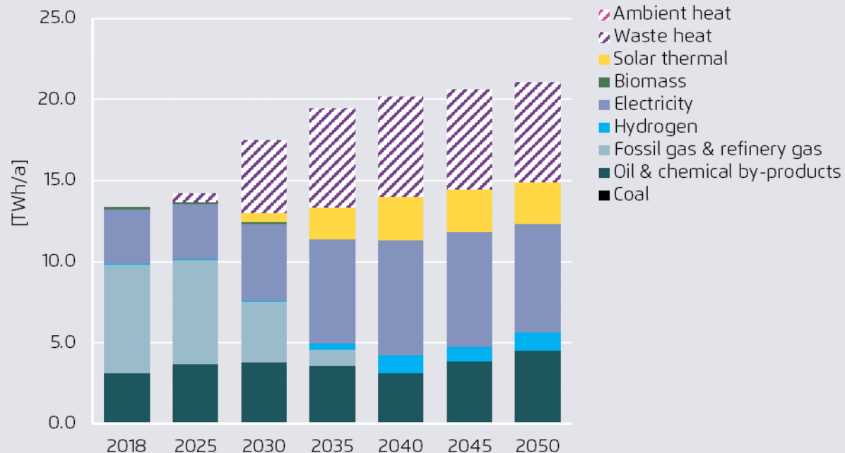
Final energy use and feedstock input in the chemical industry, Hungary
