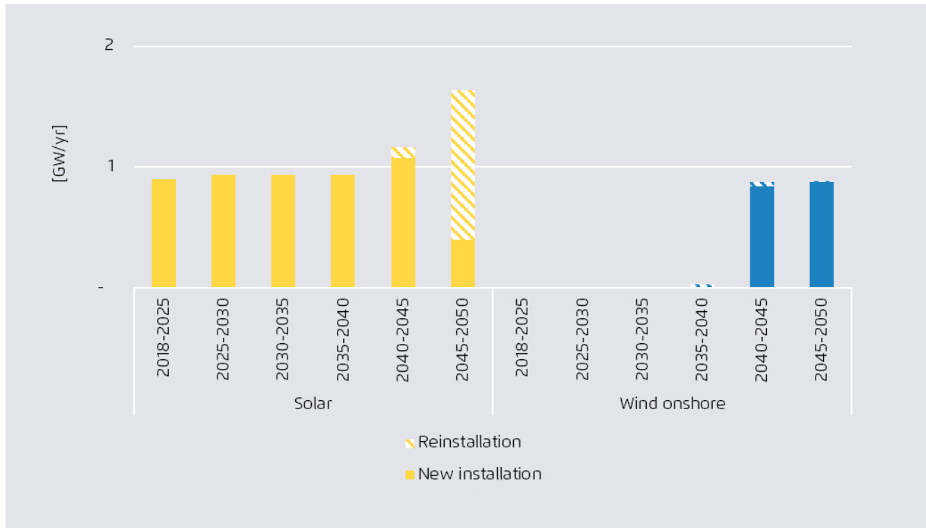
Power generation capacity installation rate per 5-year period in Hungary
