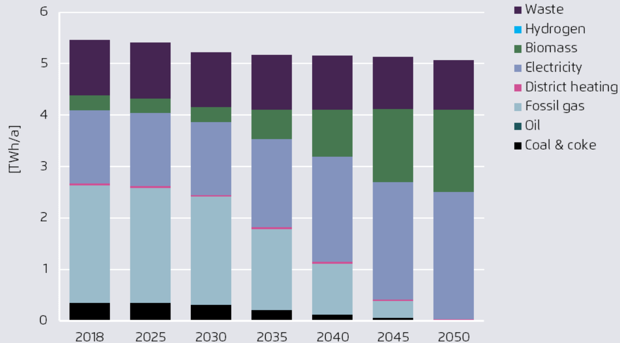
Final energy demand in the processing of non-metallic minerals, Hungary
