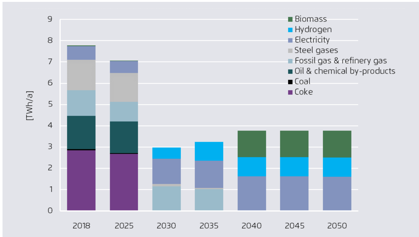
Final energy use of the steel industry, Hungary
