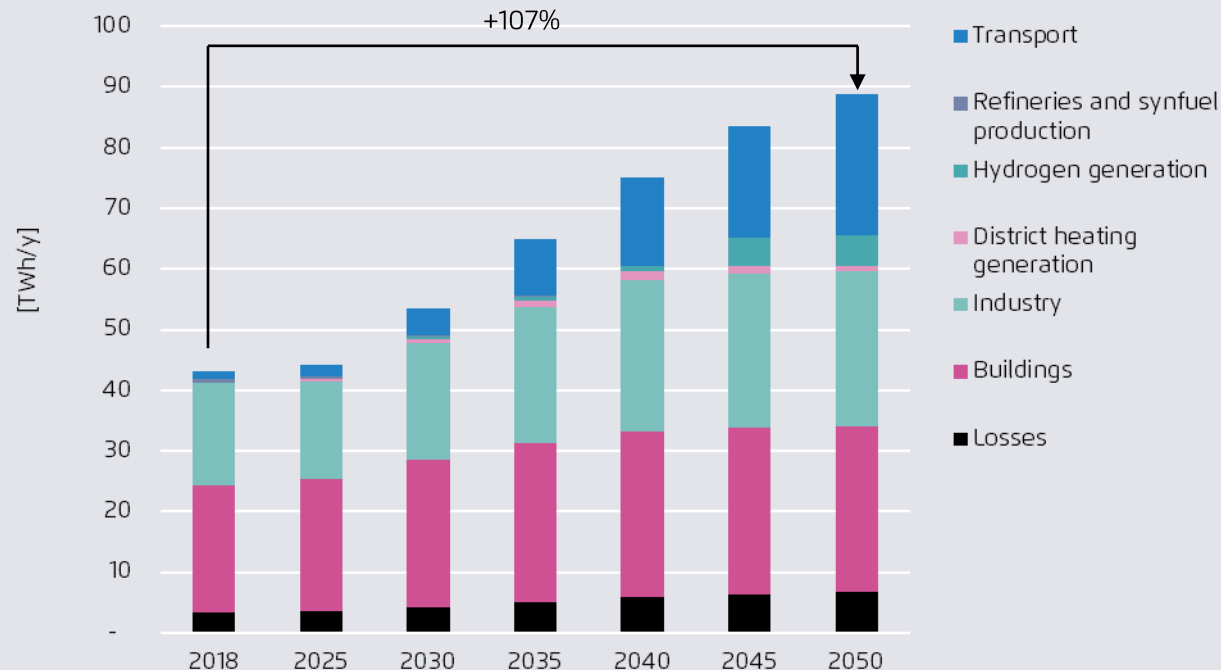
Power consumption by sector for Hungary
