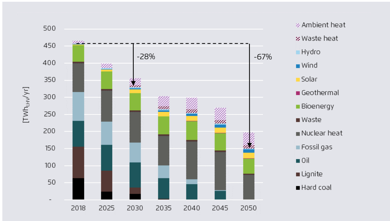
Primary energy demand* by energy source, Czech Republic
