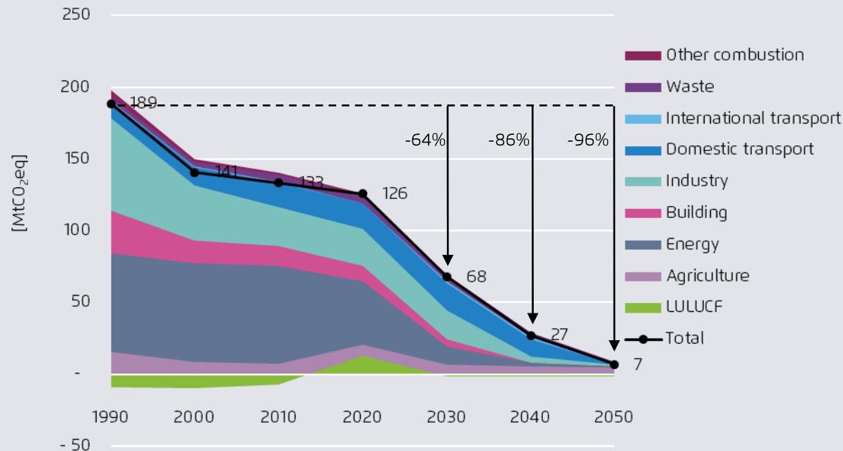
GHG emissions by sector in the Czech Republic
