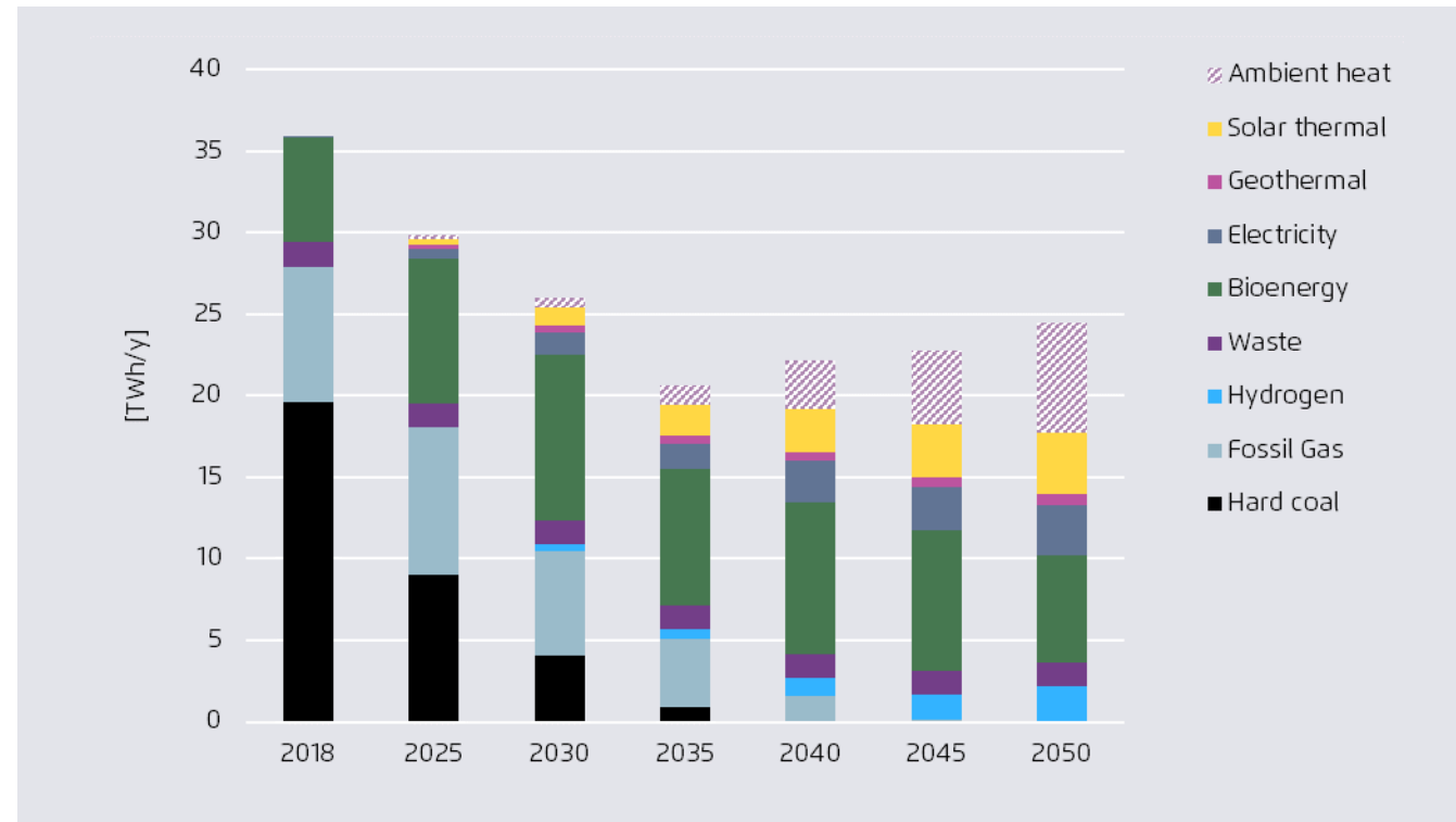
Energy input to district heating (including CHPs), Czech Republic
