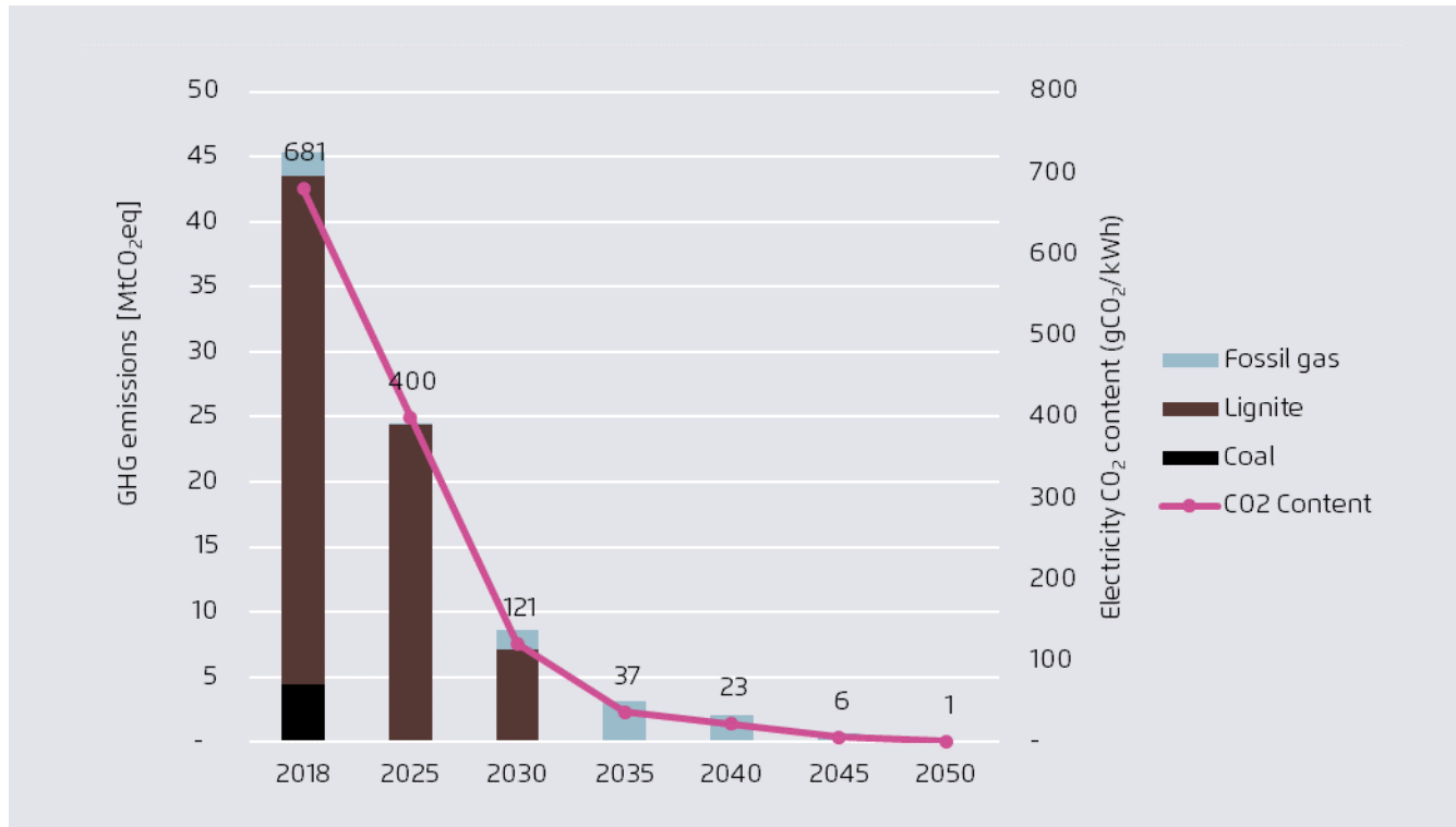
Evolution of electricity CO 2 content, Czech Republic
