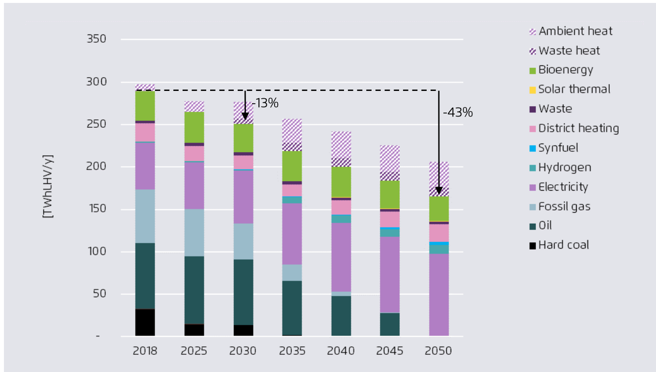
Final energy demand by energy carrier, Czech Republic
