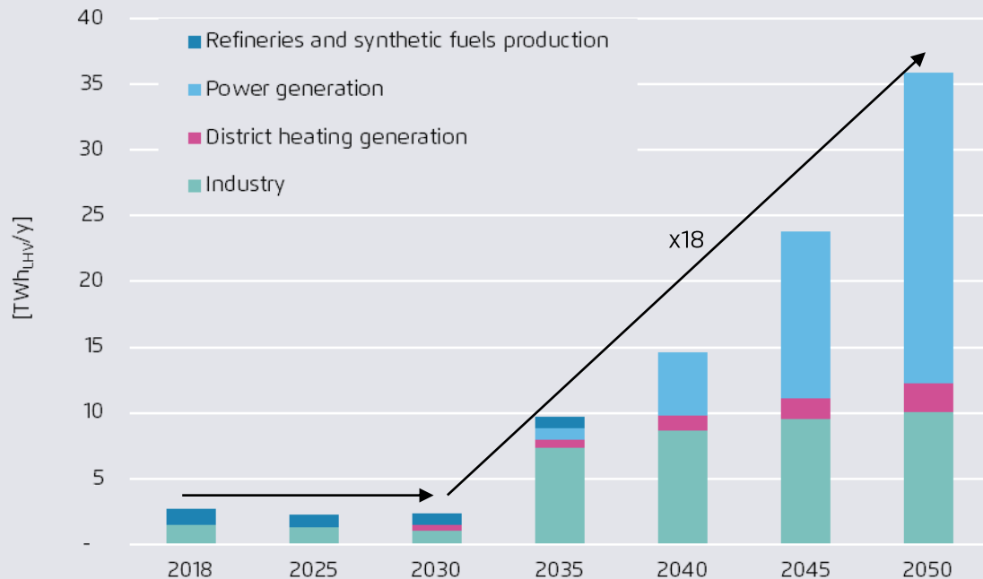
Hydrogen consumption by sector for Czech Republic
