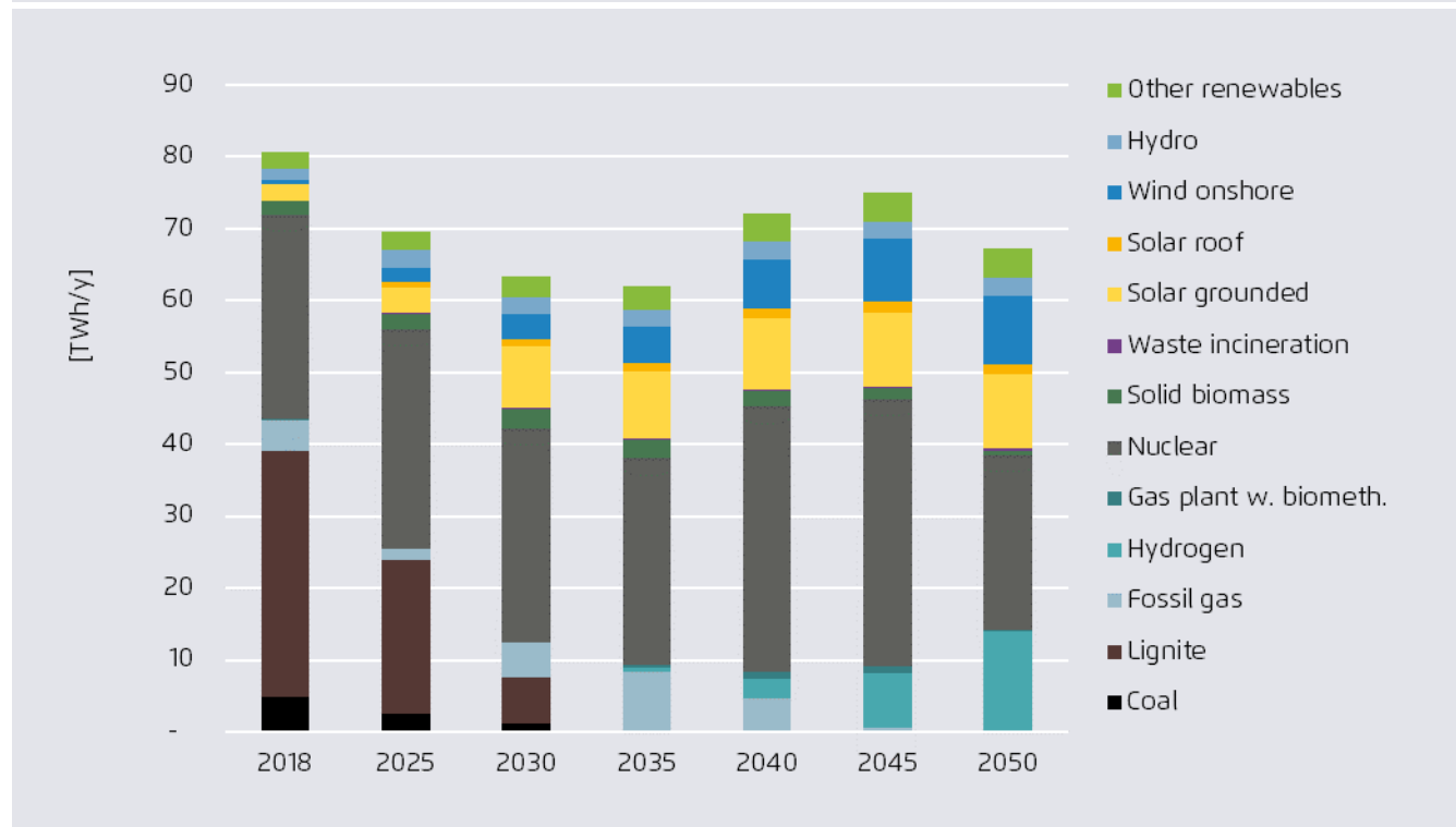
Power generation in Czech Republic
